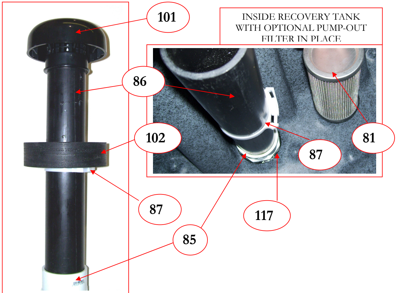
VACUUM SHUTOFF ASSEMBLY
