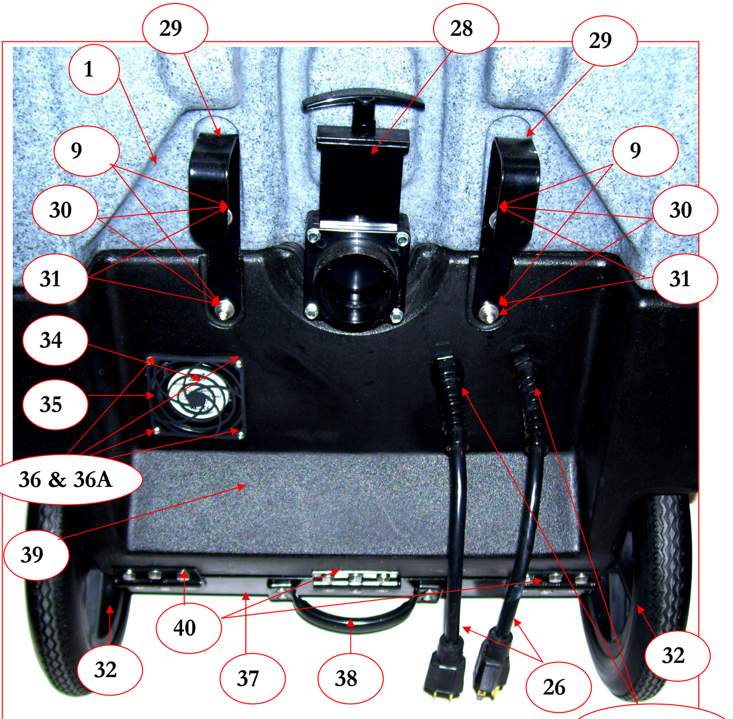
REAR VIEW – BASE, BASE SKIRT & RECOVERY TANK Shown with optional Pump-Out
